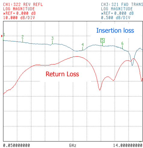
Switch Insertion Loss (Test Board minus Calibration Line Loss)
